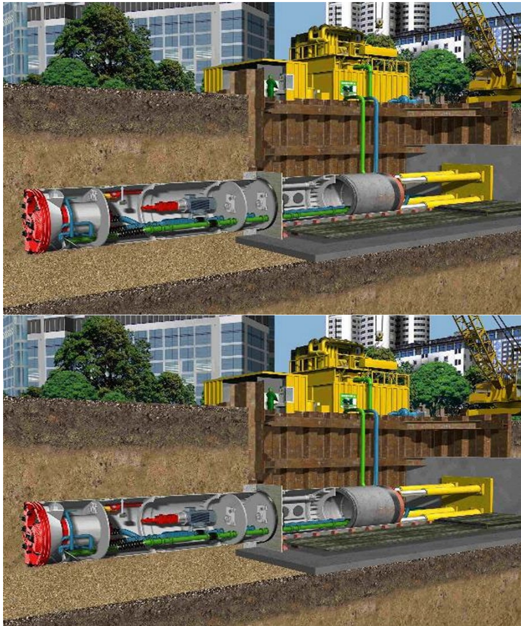
Plate 3.10: Indicative micro-tunnelling schematic
